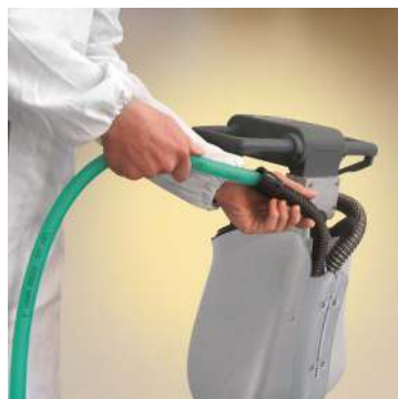
Vispa 35 B-BS Periodic cleaning of the squeegee hose to ensure efficient suction
